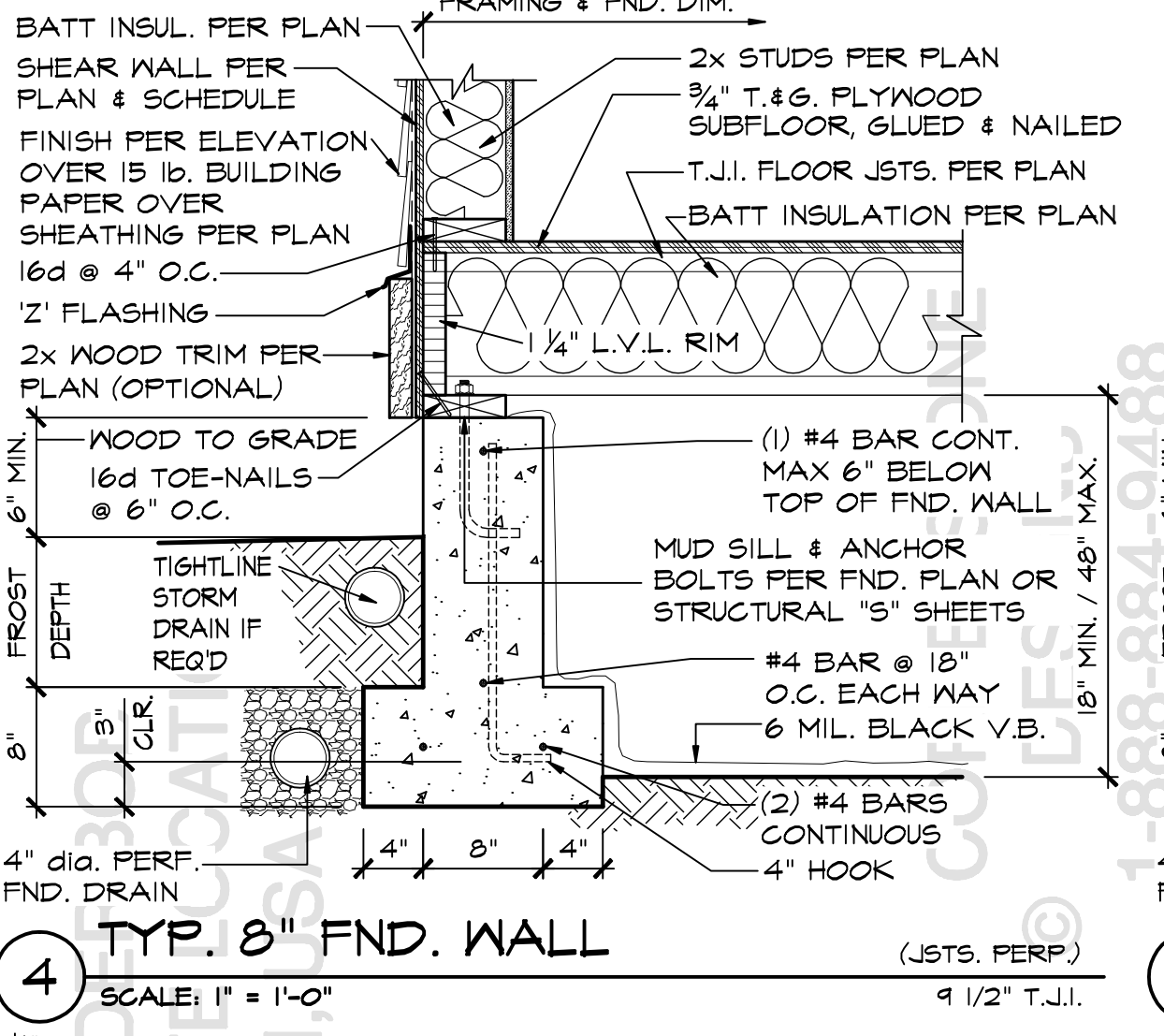
TYP. 8" FND. WALL
